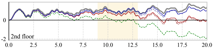
Estimated inter-story drift [cm]
