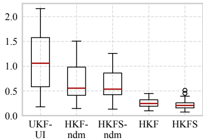
Inter-story drift RMSE [cm]
