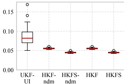
Inter-story drift RMSE [cm]
