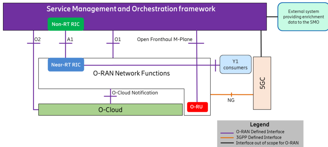
Figure 5.1-1: High Level Architecture of O-RAN
