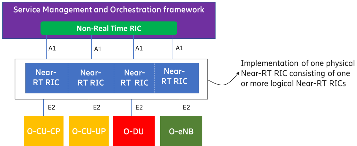
Figure A.3-2: Distributed Near-RT RIC
