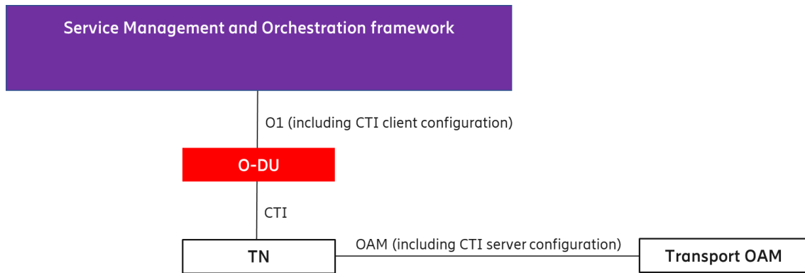
A.5-1: Simplified CTI Architecture
