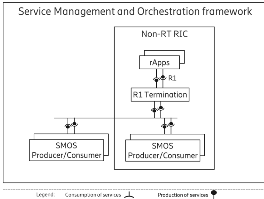
Figure 5.3.1.2.1-1: SMO architecture overview
