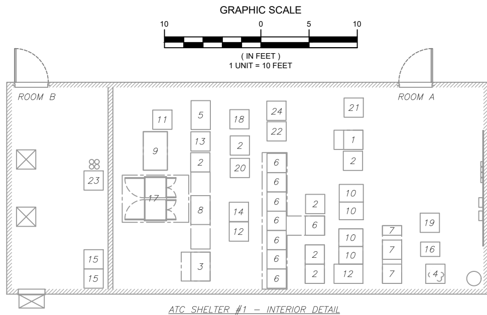
ATC SHELTER #1 - INTERIOR DETAIL
