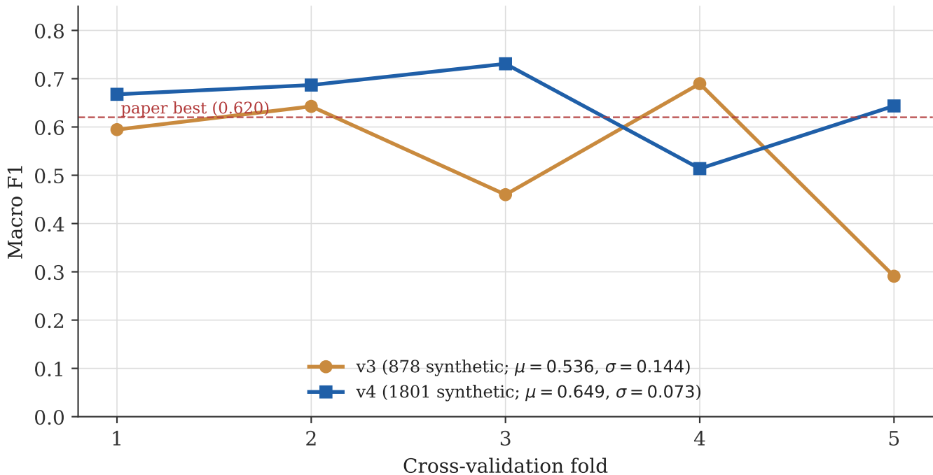
Per-fold macro F1: doubling style-anchored synthetic data halves cross-fold variance (v3 \rightarrow v4)
