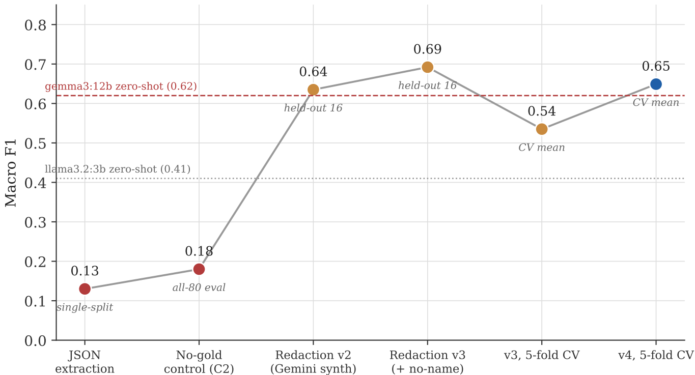
Macro-F1 across the project's development timeline
