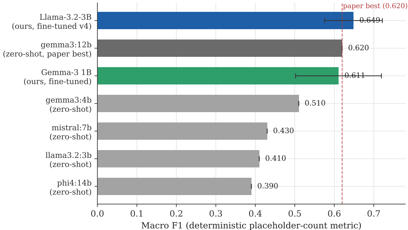
Macro-F1 across zero-shot baselines and fine-tuned models (5-fold CV mean \pm std where applicable)
