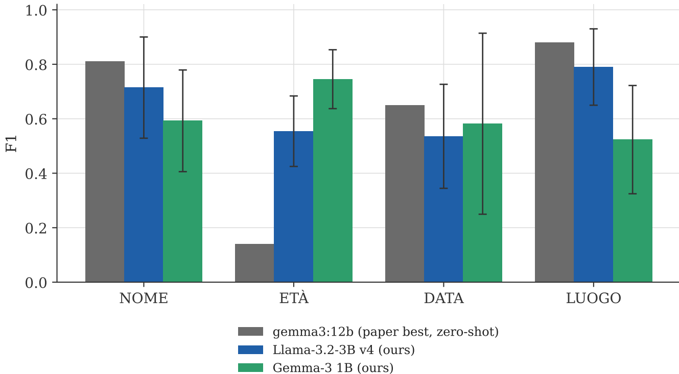
Per-category F1: fine-tuned models vs. best zero-shot baseline
