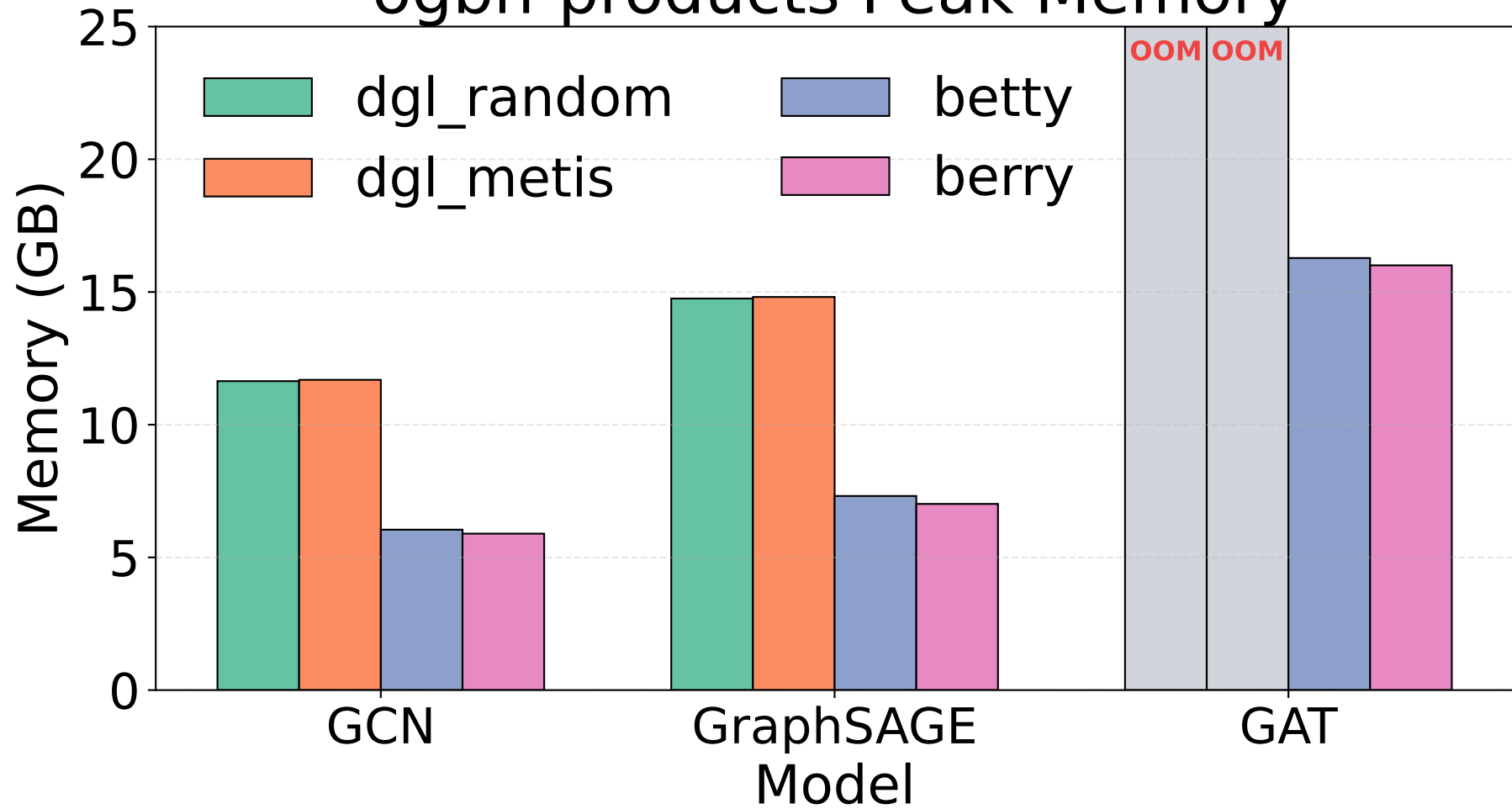
ogbn-products Peak Memory
