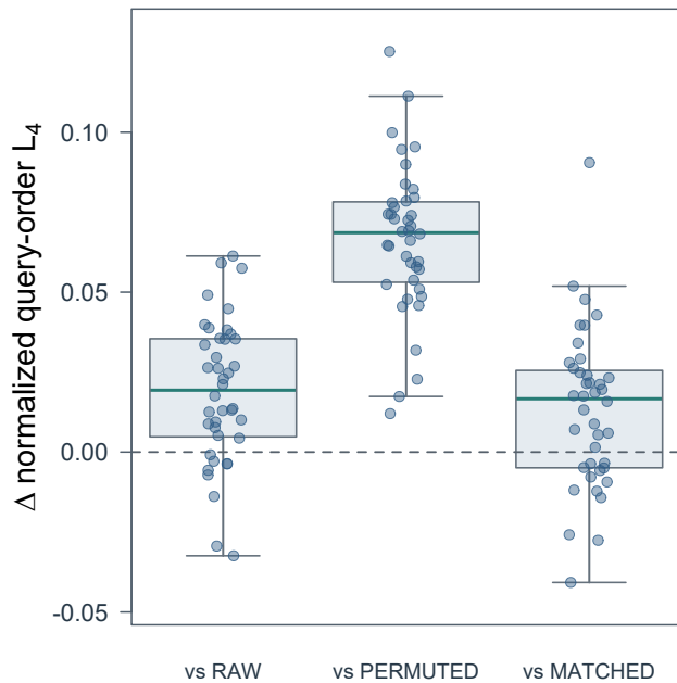
Rank acquisition
