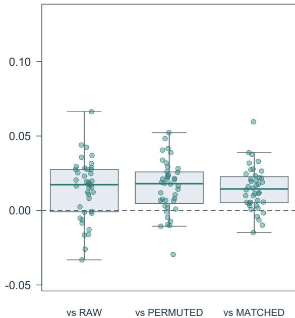
Magnitude acquisition
