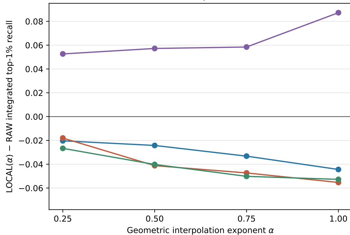
Rank acquisition
