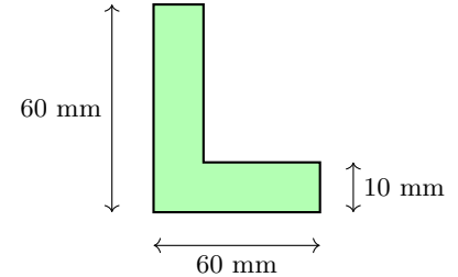
CROSS SECTION (L-TYPE)
