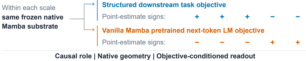
Figure 1: Study design. Native geometry and a selected causal component are reconstructed independently within each scale. The same scale-local contrast is read under downstream and pretrained objectives. Arrows indicate study order, not a continuous scaling law or shared plane identity.
