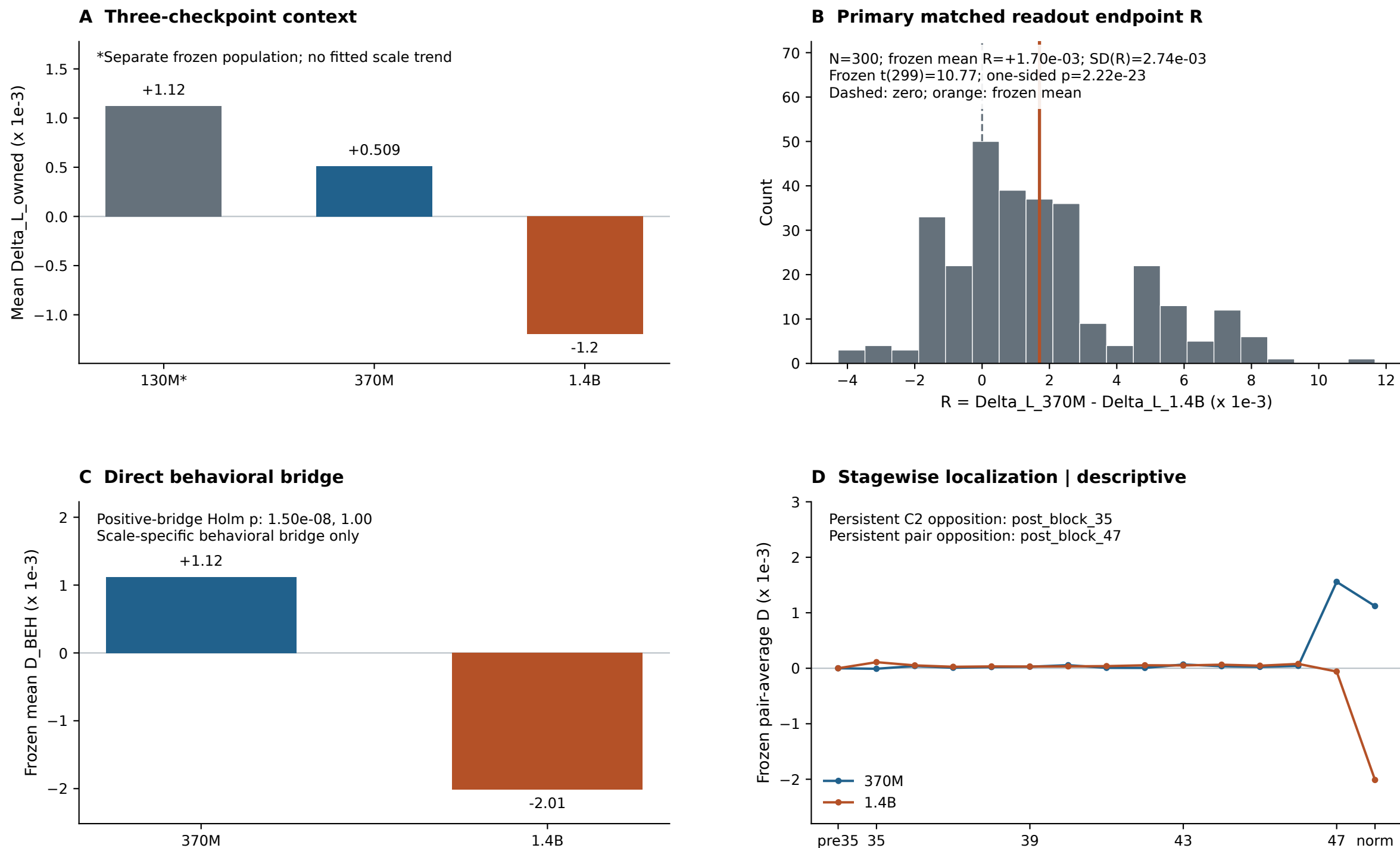
Figure 5 | Downstream readout reversal despite causal-role recurrence
