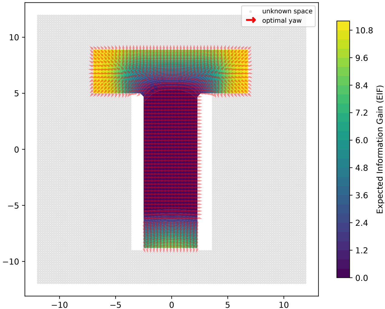
Expected Information Field (with Optimal Yaw)
