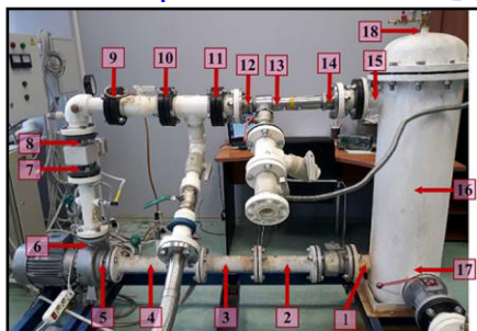
Fig. 15a. Cavitational iWET water installation with measurement points.
