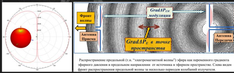
Fig.2a. Longitudinal non-shock etheric “Electromagnetic wave” ( V = C ).
