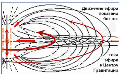
Fig. 6. Etheric double toroidal vortex of the stellar or Galactic type, including Quasars. On the right is a diagram of a toroid.
