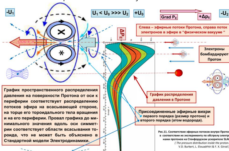
Fig. 11. Conformity of the experiment SLAC and the toroidal ring with Spin-Jet.
