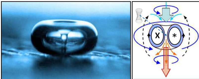
Fig. 17. Crim LJ Physique, V.40, 285, 1979., KP and the Etherodynamic Model of KP.
