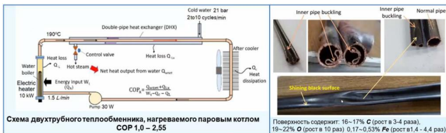
Fig. 22. Double-pipe Cavitation Reactor - left. Deformation of the internal reactor pipes - on the right.
