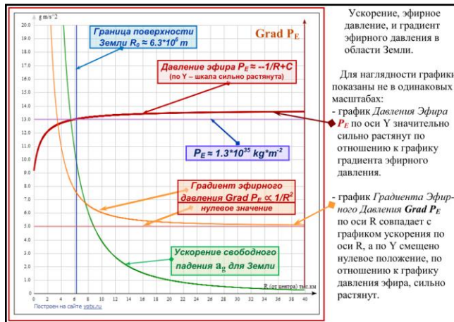
Fig. 9. Graphs of Ether Pressure, Ether Pressure Gradient, and accelerations in the region of the Earth's surface inside and outside it. (The blue vertical line is the boundary of the Earth's surface).
