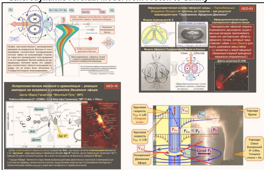
Fig. 0. Review of applications of the etherodynamic model to various physical processes.
