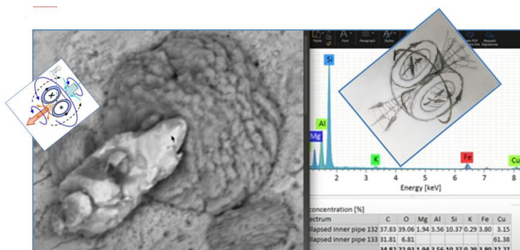
Fig. 19. Spin-Jet of toroidal structure of "cavitation bubble" from materials of R. Grinier.
