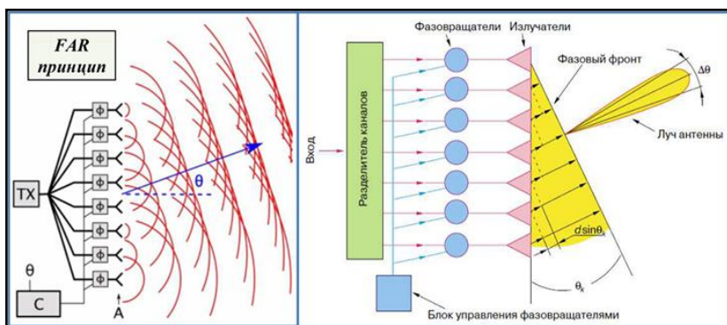
Fig.2b. The principle of radiation and control of the direction of propagation and shape ether-dynamic wave by changing the phase for each radiation element of the FAR antenna.
