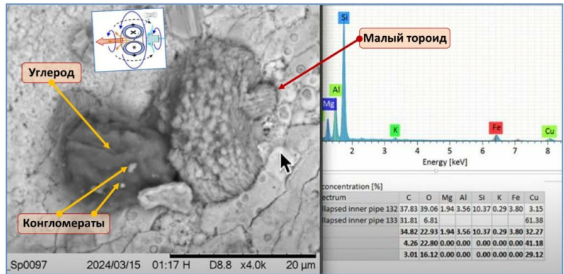
Fig. 21. Emission of carbon by a cavitation toroid and conglomerates with the composition specified in table.
