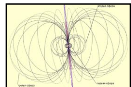
Fig.10. Ethereal Galactic fractal vi hr
