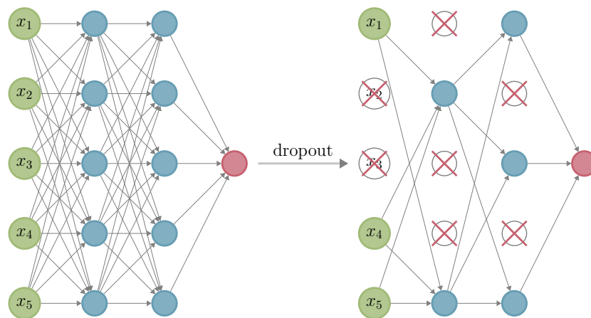
Figure 2.7: Dropout during training. For each iteration, a random subset of neurons (shown crossed out) is dropped, effectively training a different sub-network at each step.
