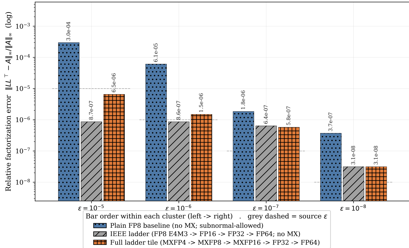
Ladder mode at tile granularity, N = 32768 , NB = 2048
