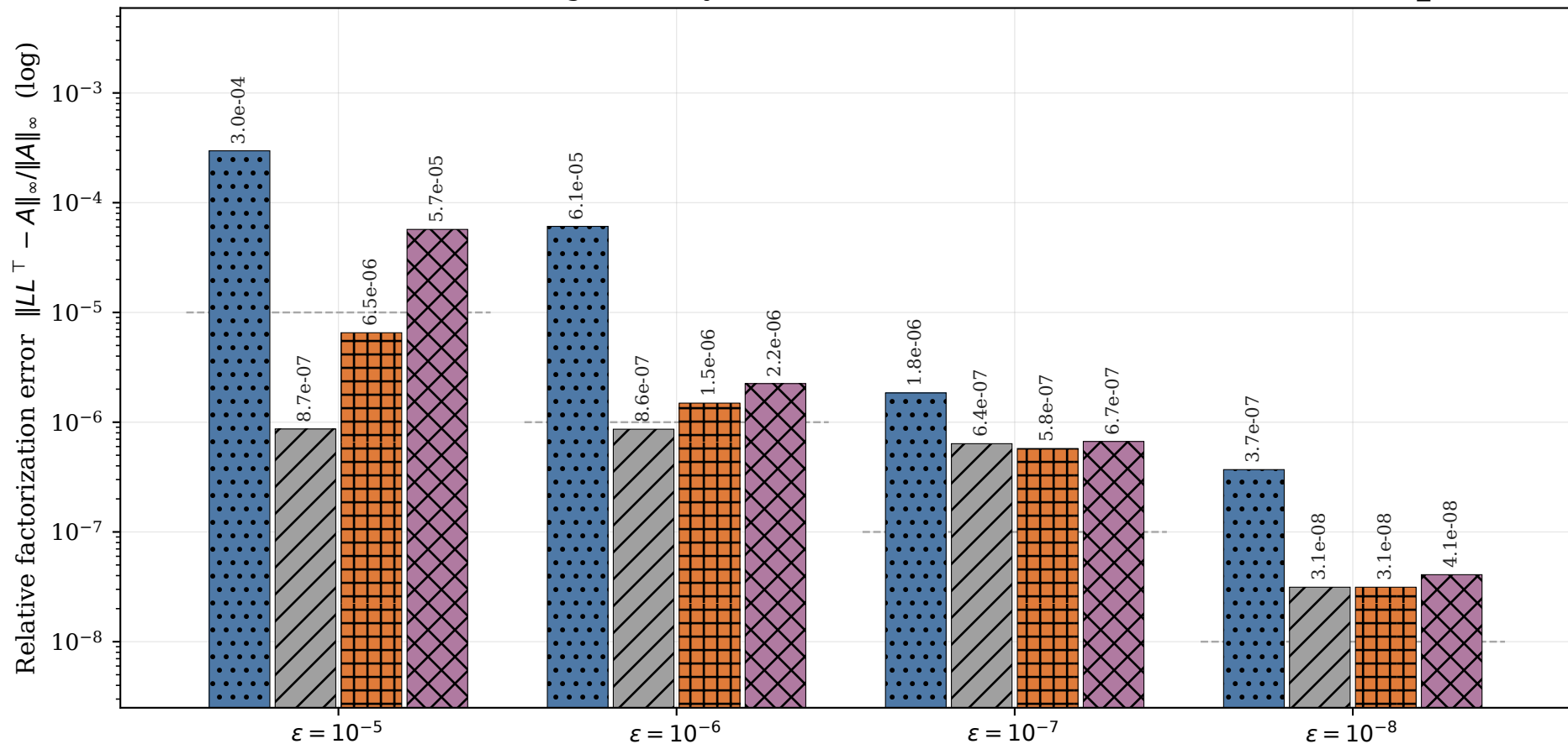
Ladder mode at tile + vec1D-32 granularity, N = 32768, NB = 2048 (32k vec1d32 uses ladder_rerun GU)
