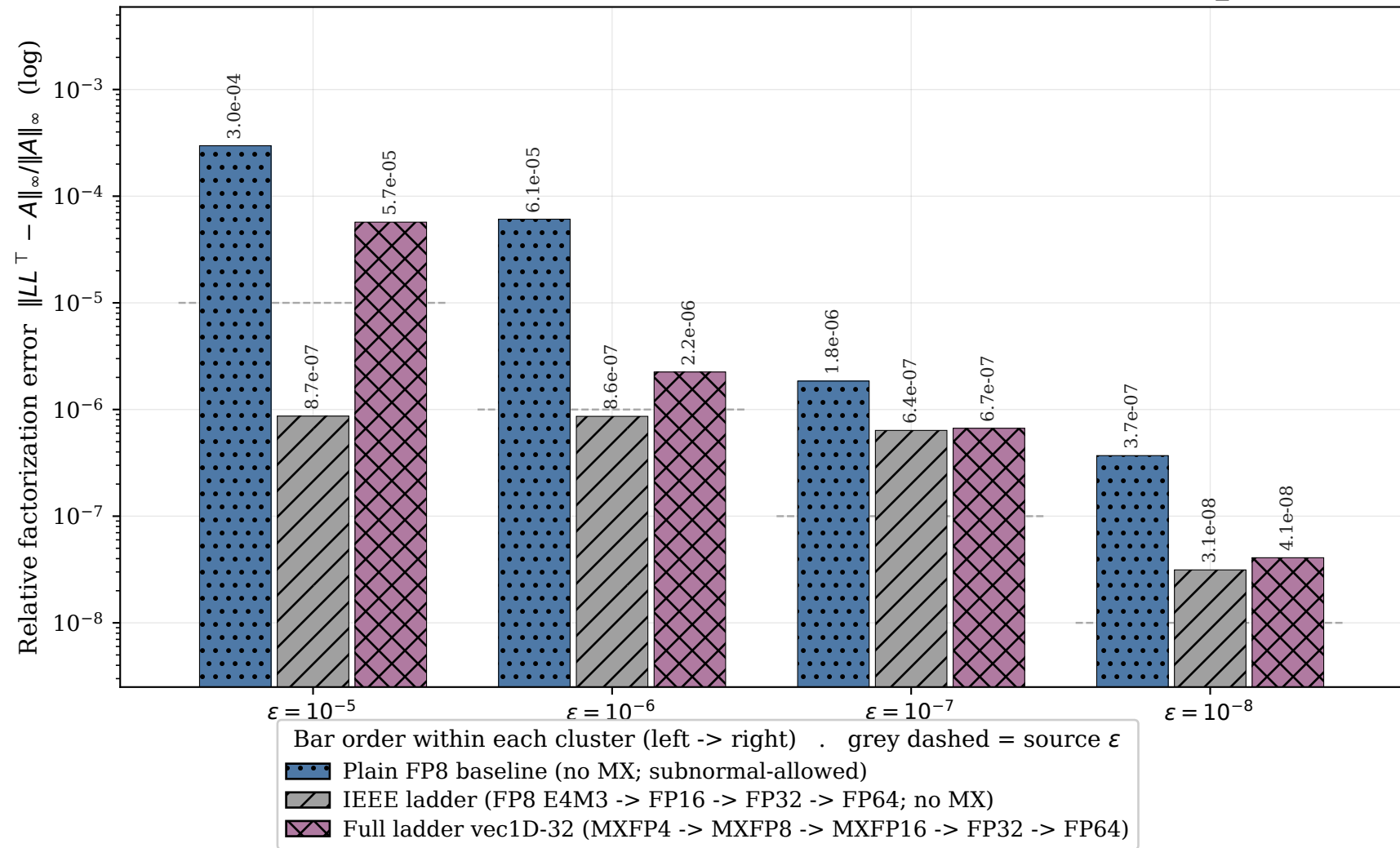
Ladder mode at vec1D-32 granularity, N = 32768, NB = 2048 (32k uses ladder_rerun GU)
