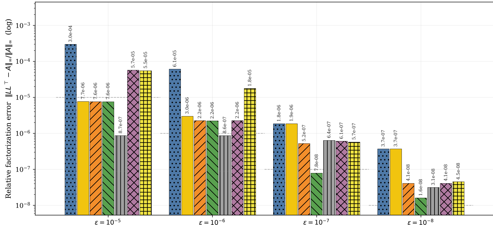
Progressive MX scaling at N=32768 (MX-native storage, 1×32 row groups)
