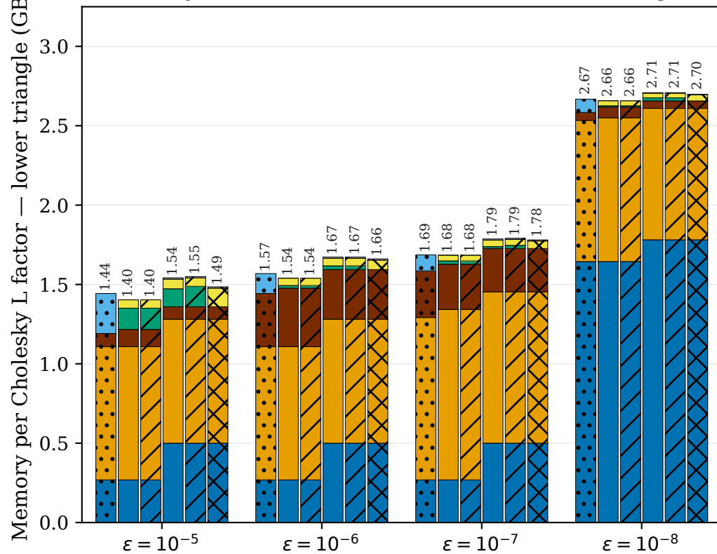
Memory (ladder, N=32768, nb=2048, lower triangle)
