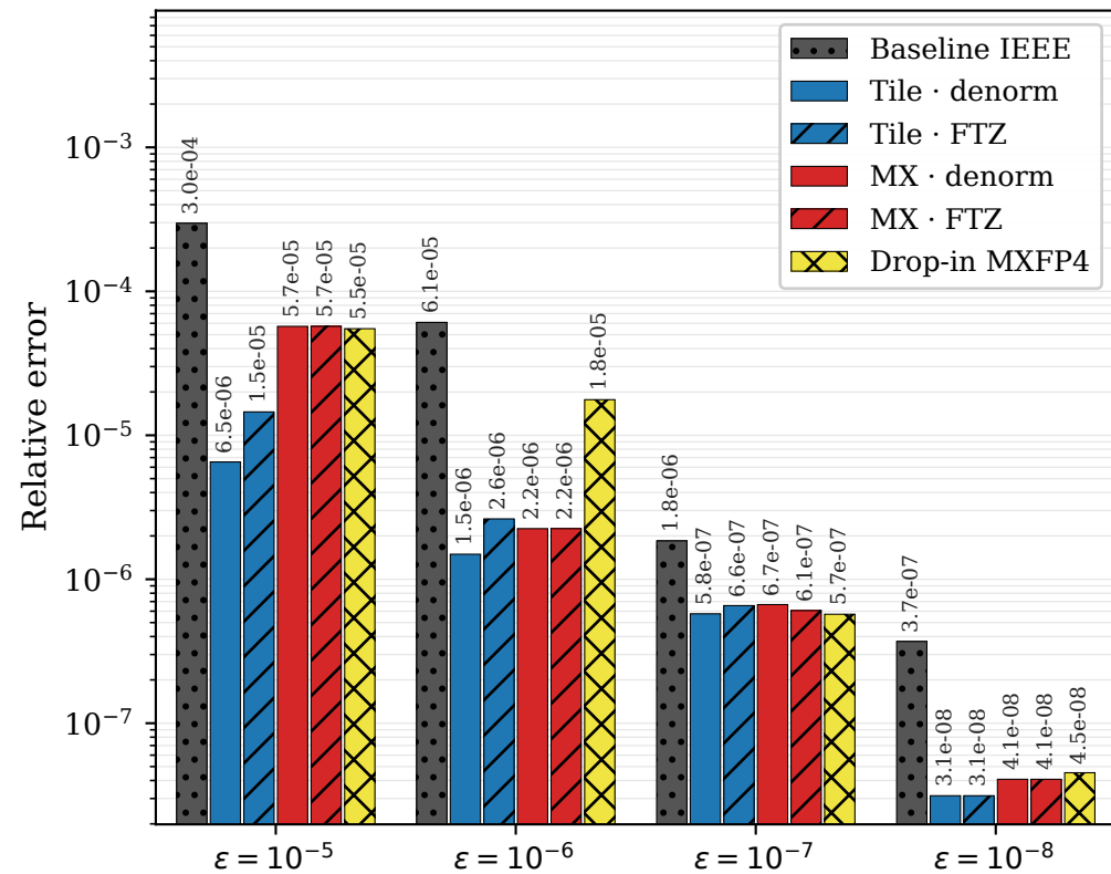
Error (ladder, N=32768, nb=2048)
