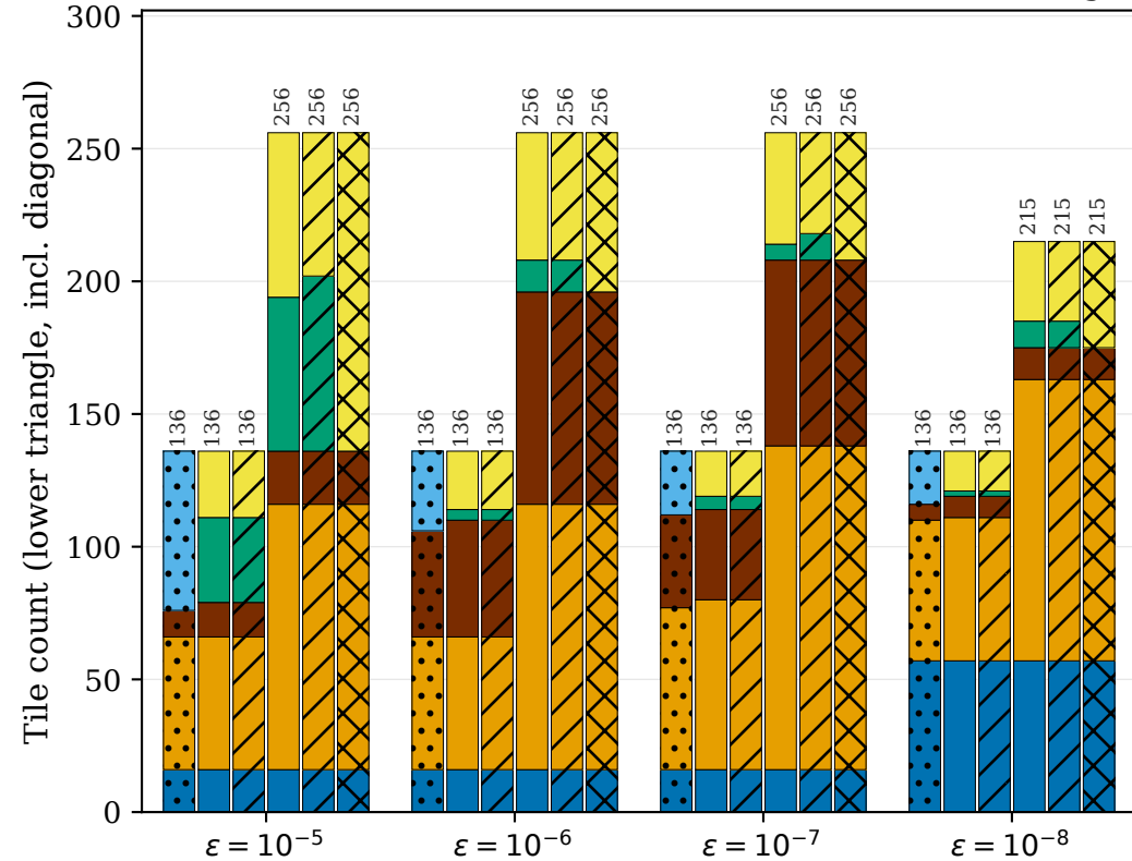
Tile allocation (ladder, N=32768, nb=2048, lower triangle)
