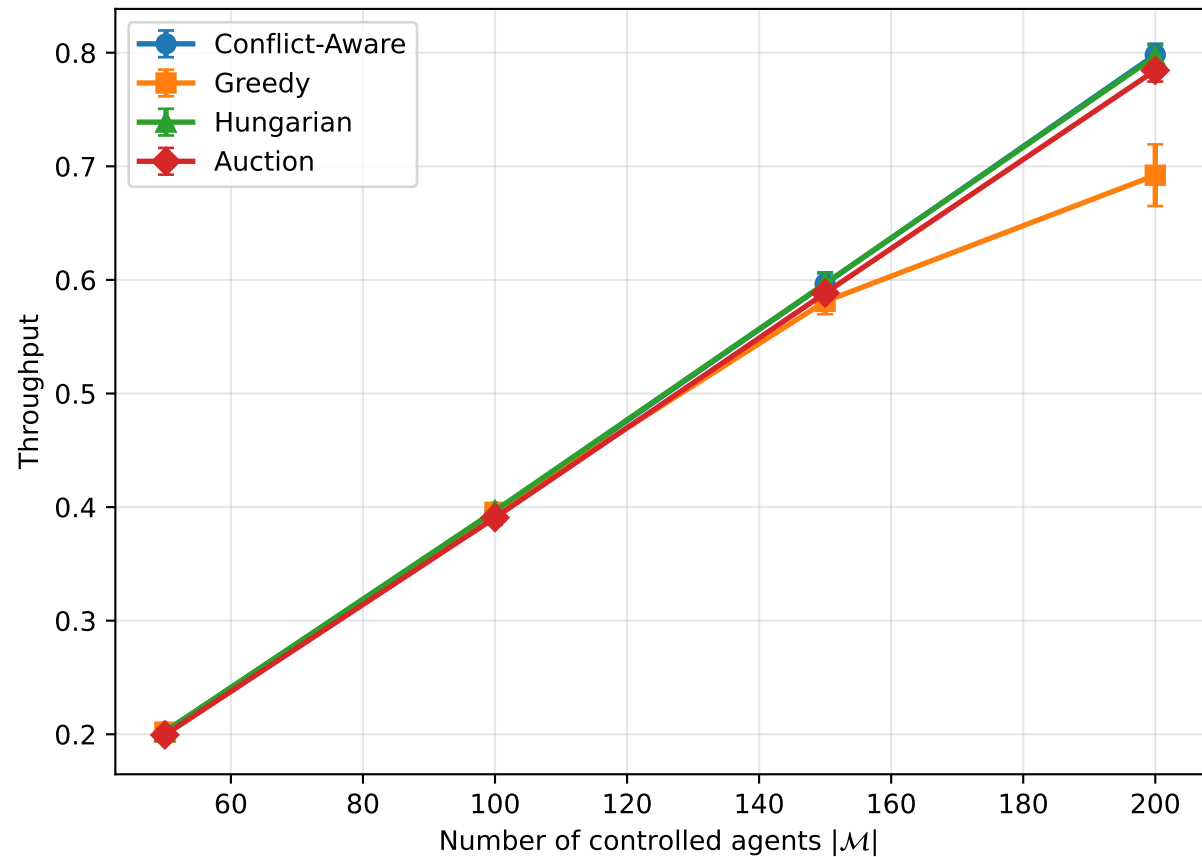
warehouse-10-20-10-2-2 ( r_{fov} = 3, r_{safe} = 1 )
