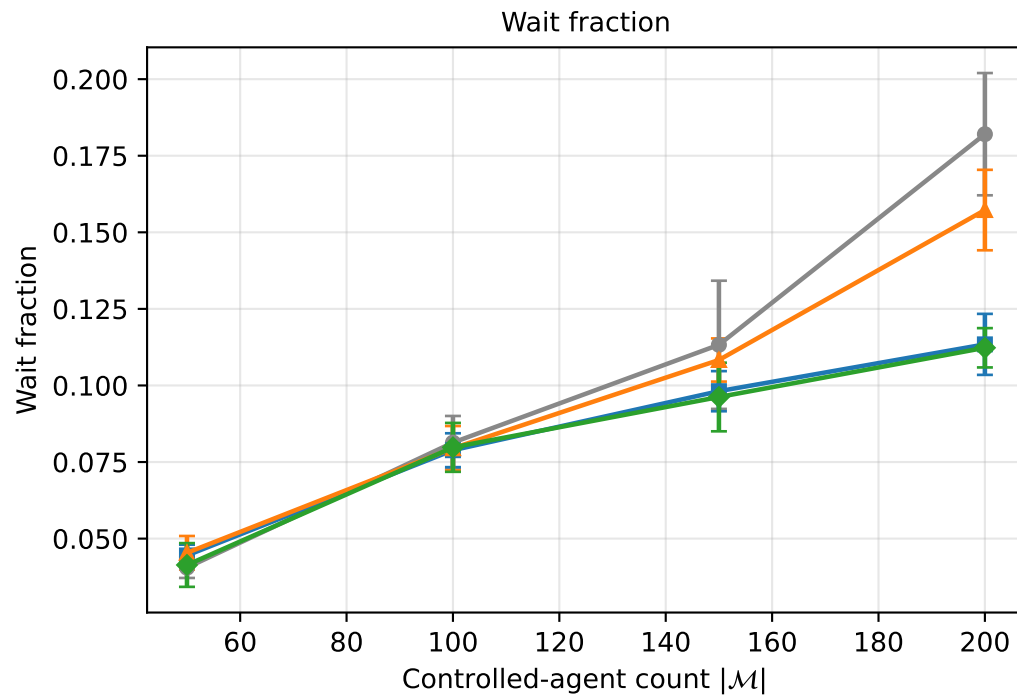
Task-allocator comparison — warehouse-10-20-10-2-2 (fov3_safe1_v3)
