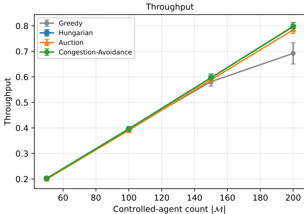
Task-allocator comparison — warehouse-10-20-10-2-2 (fov3_safe1_v3)
