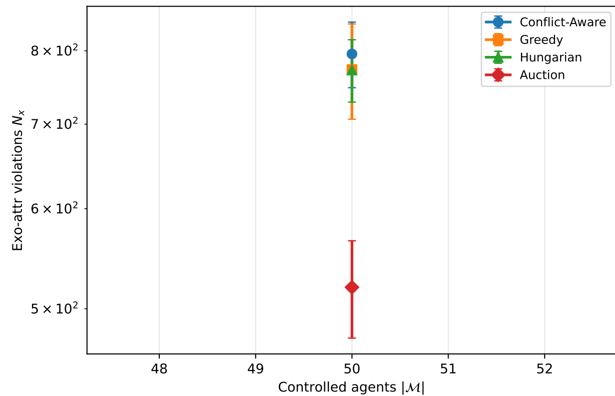
random-64-64-10: allocator detail @ ( r_{fov} = 3 , r_{safe} = 1 )
