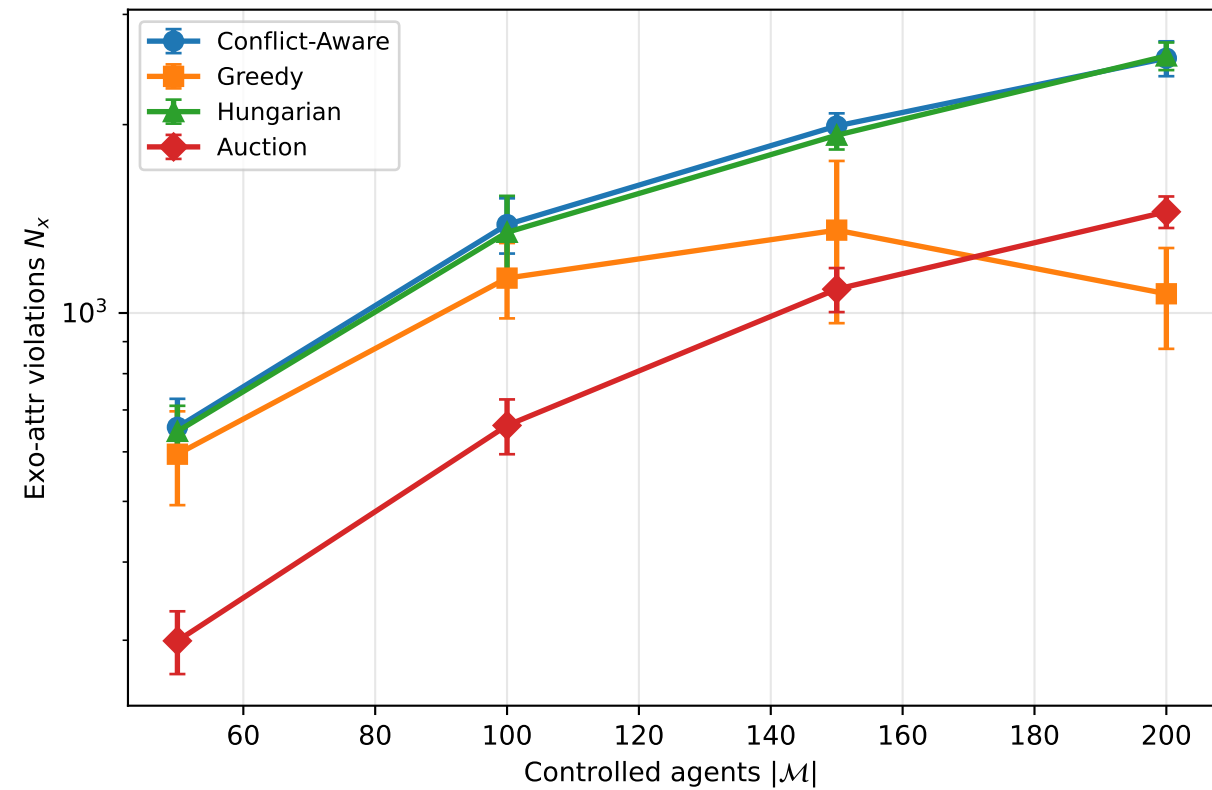
warehouse-10-20-10-2-2: allocator detail @ ( r_{fov} = 3 , r_{safe} = 1 )
