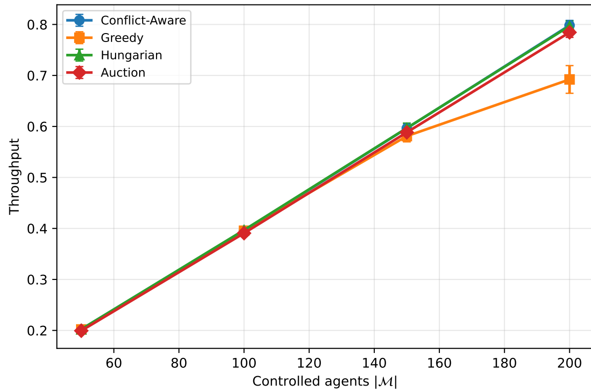
warehouse-10-20-10-2-2: allocator detail @ ( r_{fov} = 3 , r_{safe} = 1 )
