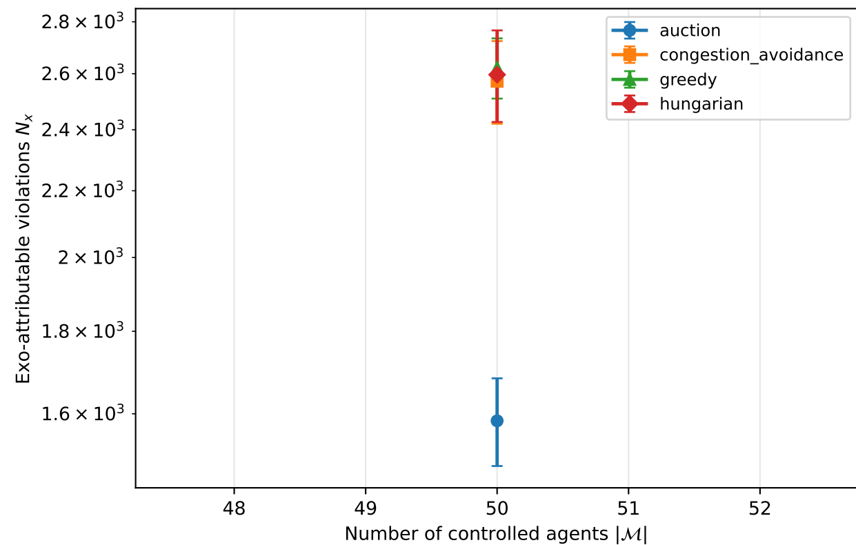
random-64-64-10: allocator comparison @ ( r_{fov} = 4, r_{safe} = 2 ) [v2]
