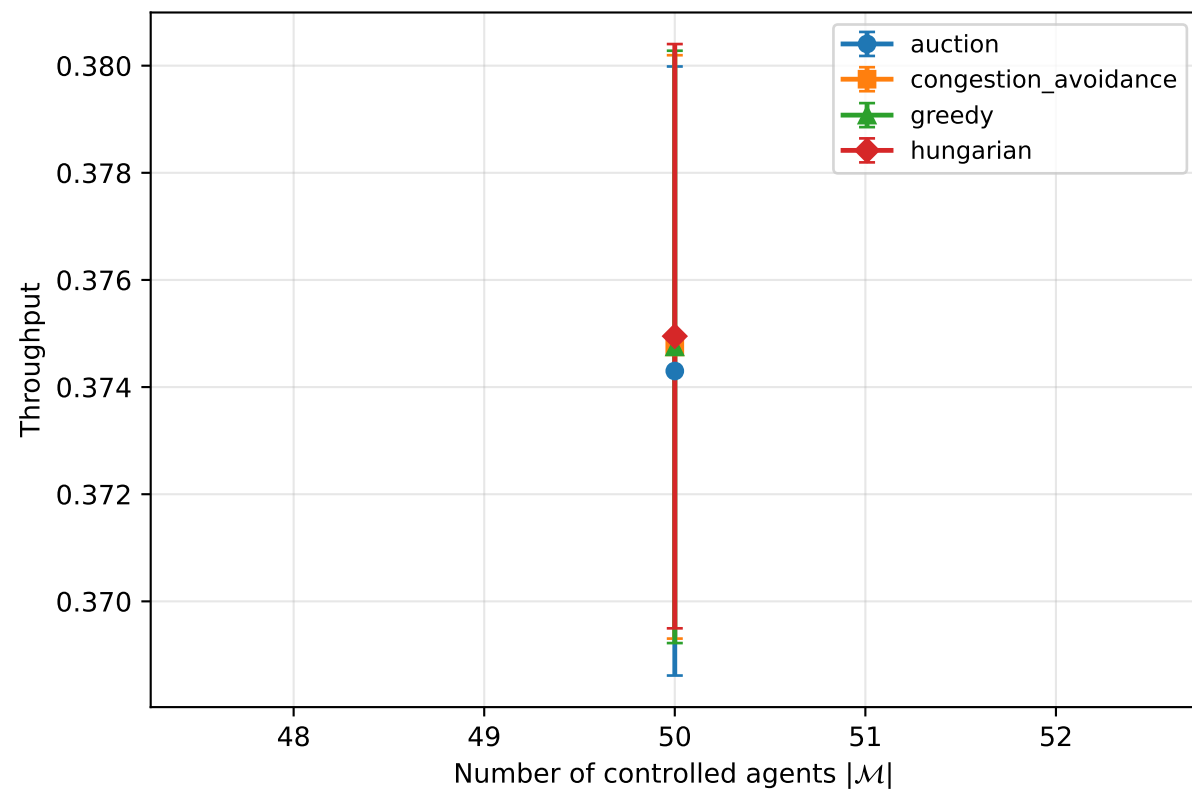
random-64-64-10: allocator comparison @ ( r_{fov} = 4, r_{safe} = 2 ) [v2]
