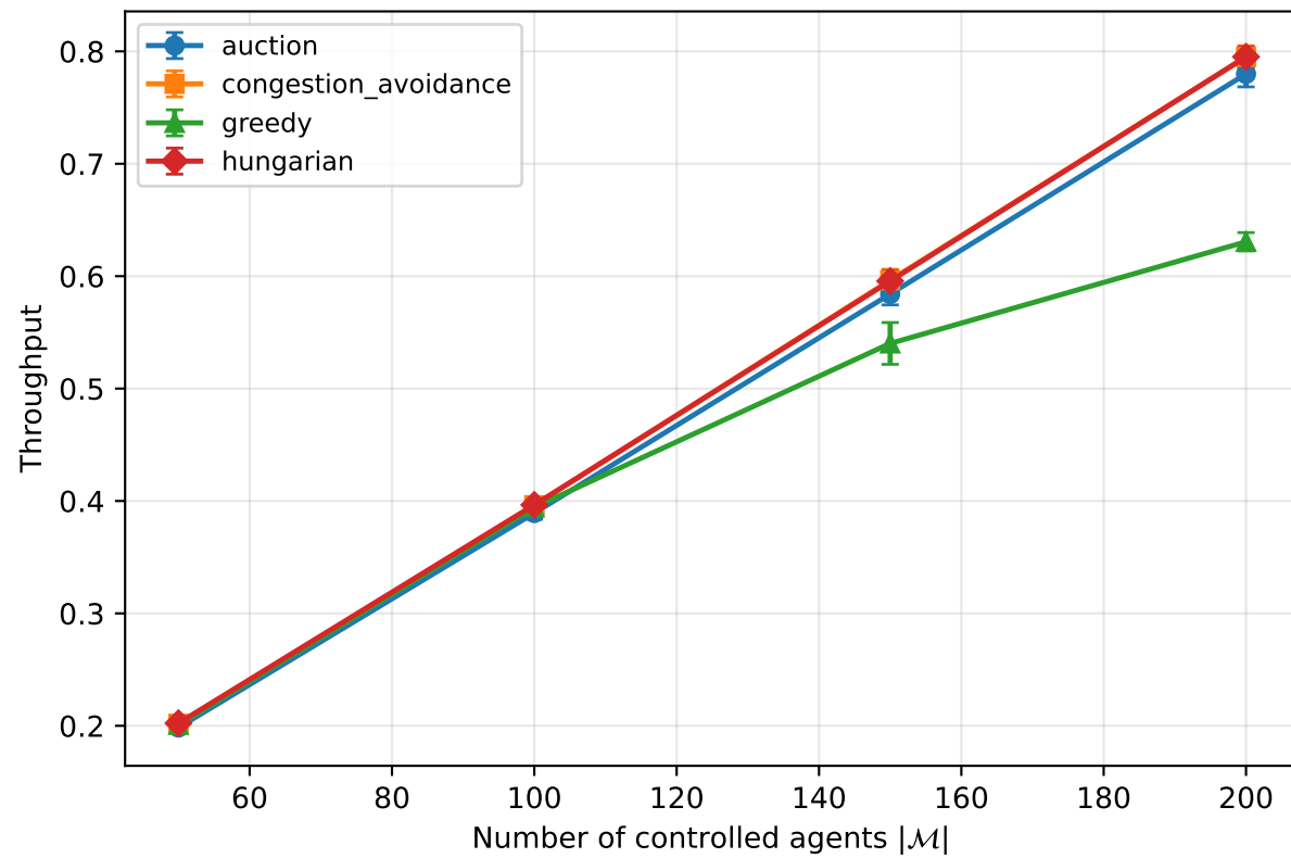
warehouse-10-20-10-2-2: allocator comparison @ ( r_{fov} = 4 , r_{safe} = 2 ) [v2]
