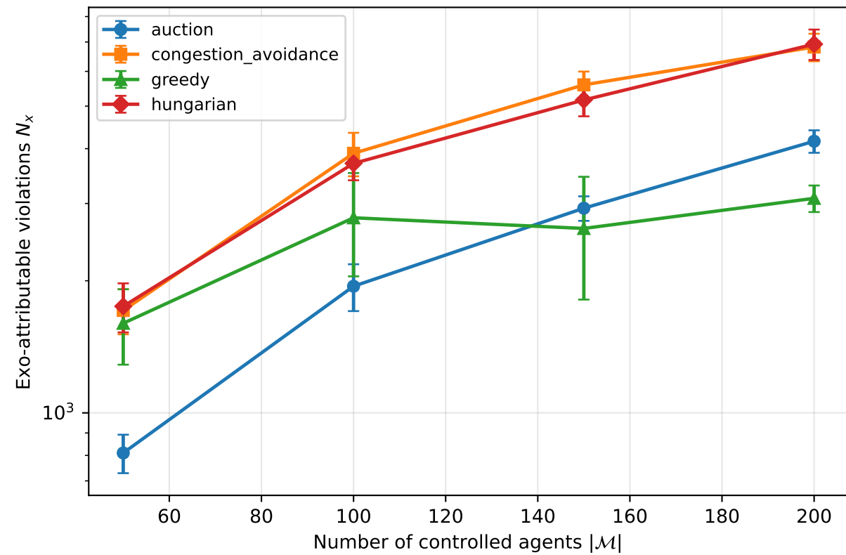
warehouse-10-20-10-2-2: allocator comparison @ ( r_{fov} = 4 , r_{safe} = 2 ) [v2]
