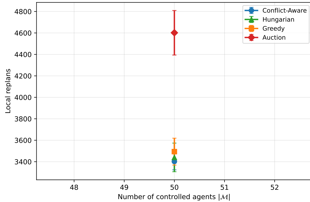
random-64-64-10: allocator comparison @ ( r_{fov} = 3 , r_{safe} = 1 )
