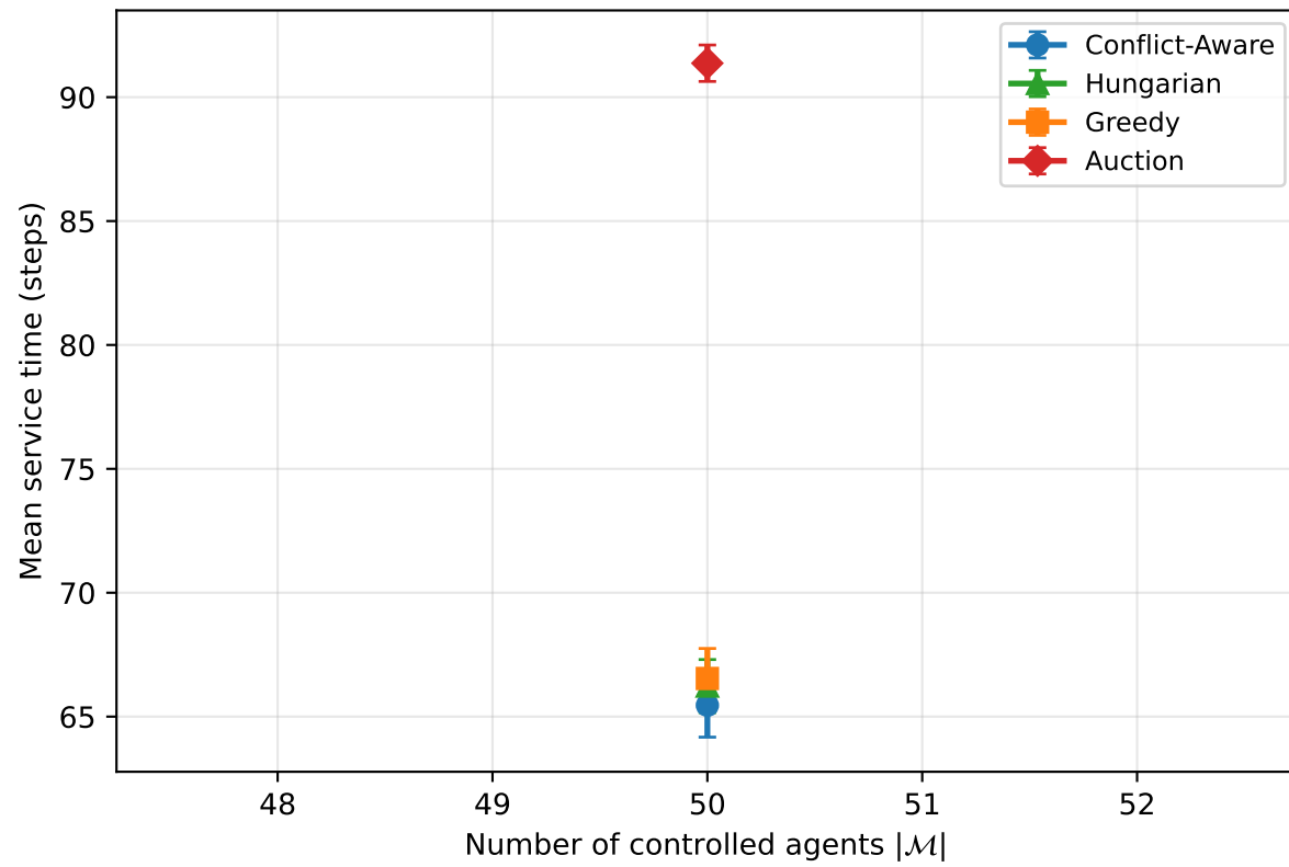
random-64-64-10: allocator comparison @ ( r_{fov} = 3 , r_{safe} = 1 )
