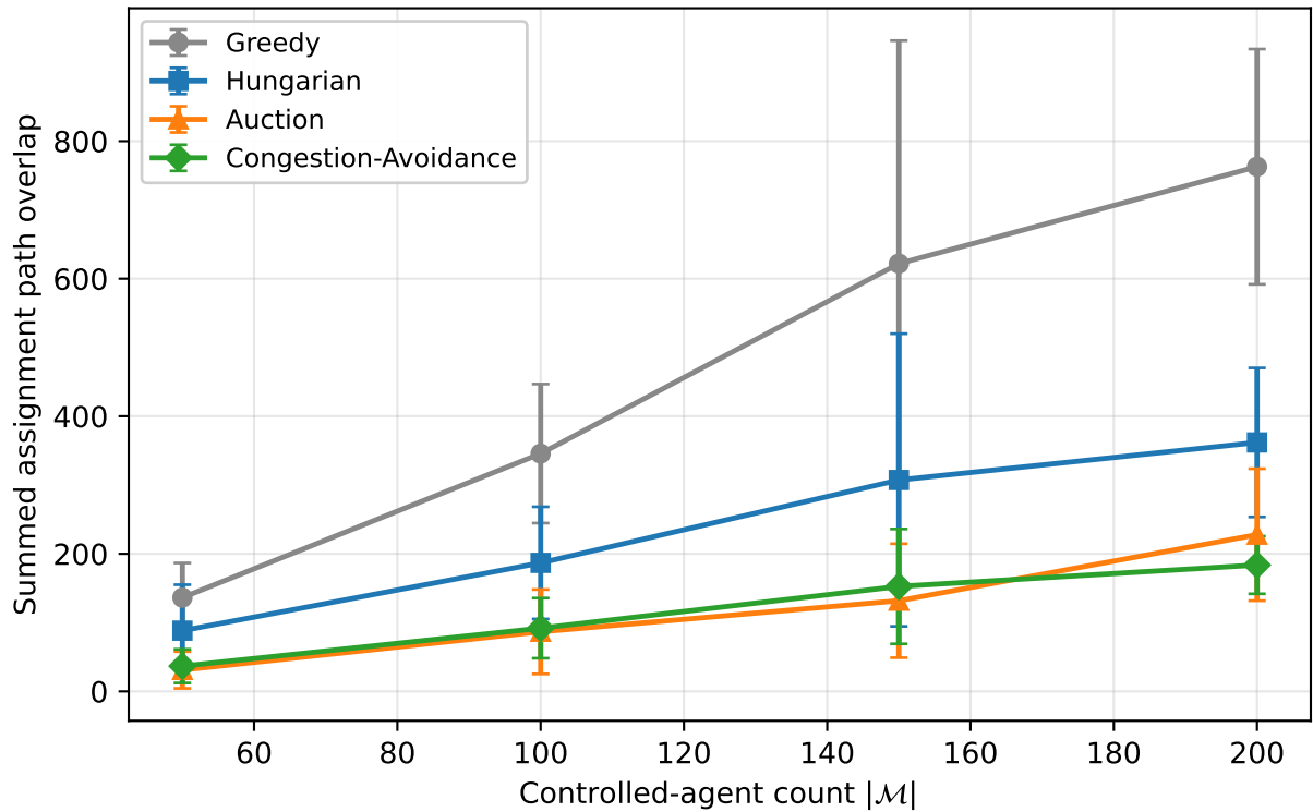
Assignment path overlap by allocator (lower = easier MAPF instance) — fov3_safe1_v3
