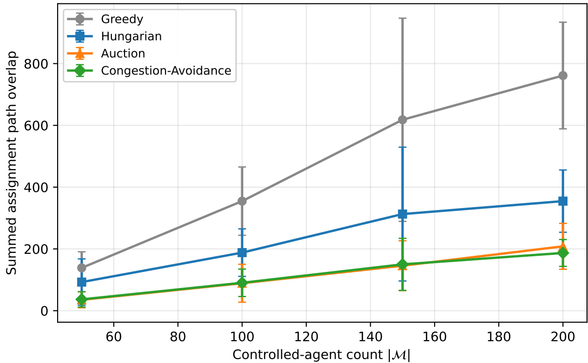
Assignment path overlap by allocator (lower = easier MAPF instance) — fov4_safe2_v2
