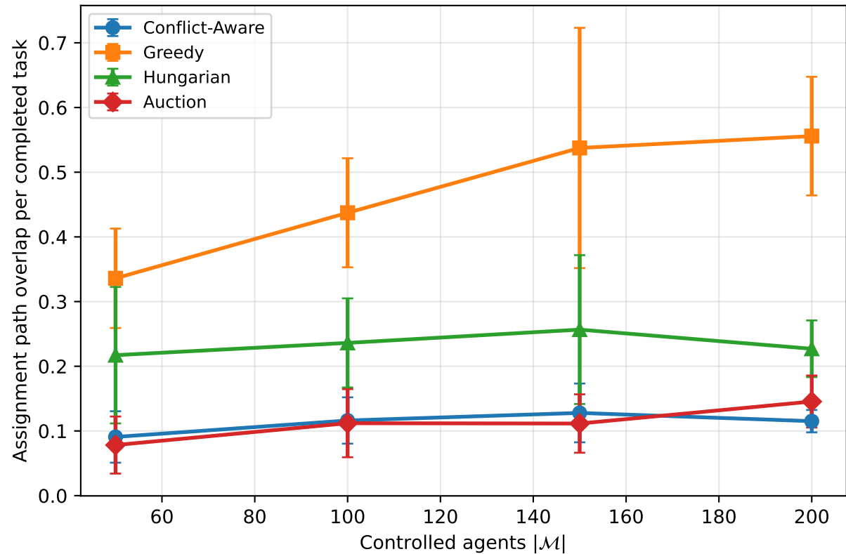
warehouse-10-20-10-2-2
