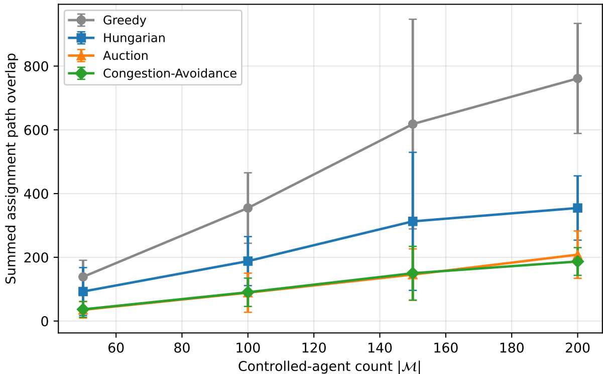
Assignment path overlap by allocator (lower = easier MAPF instance)
