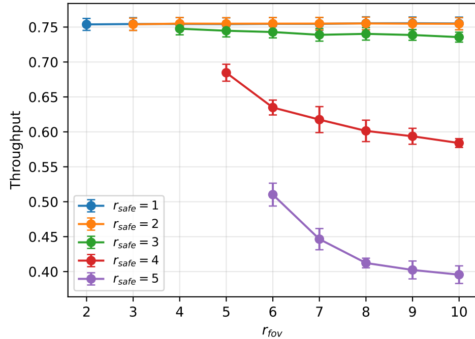
random-64-64-10: Throughput vs r_{fov}
