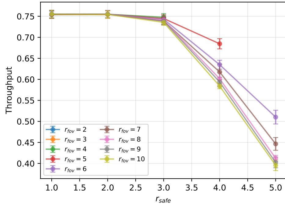
random-64-64-10: Throughput vs r_{safe}
