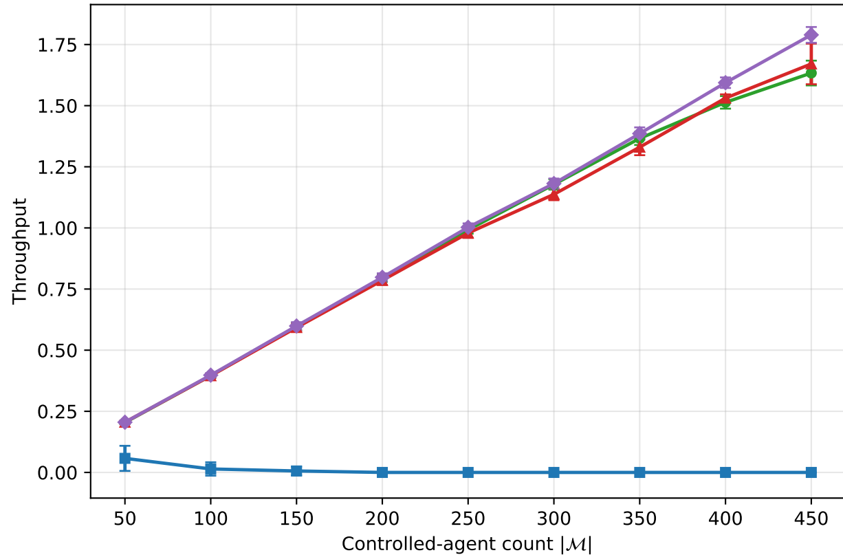
warehouse-10-20-10-2-2
