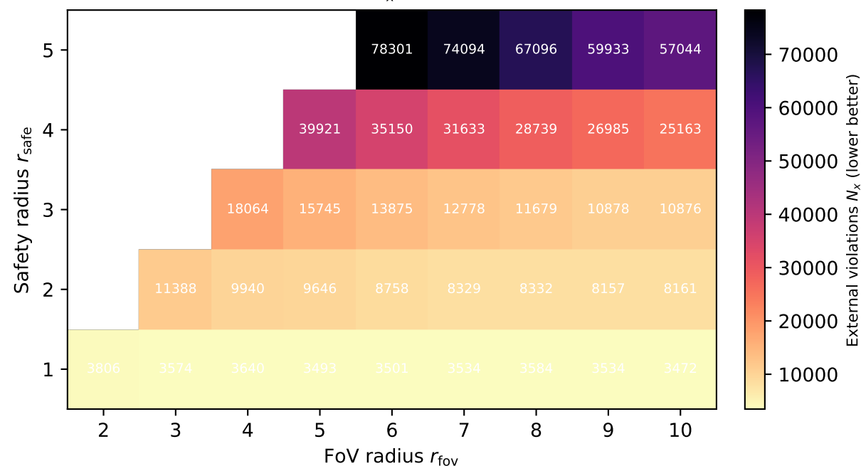
External violations N_x — random-64-64-10
