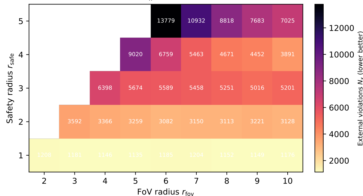
External violations N_x — warehouse-10-20-10-2-2
