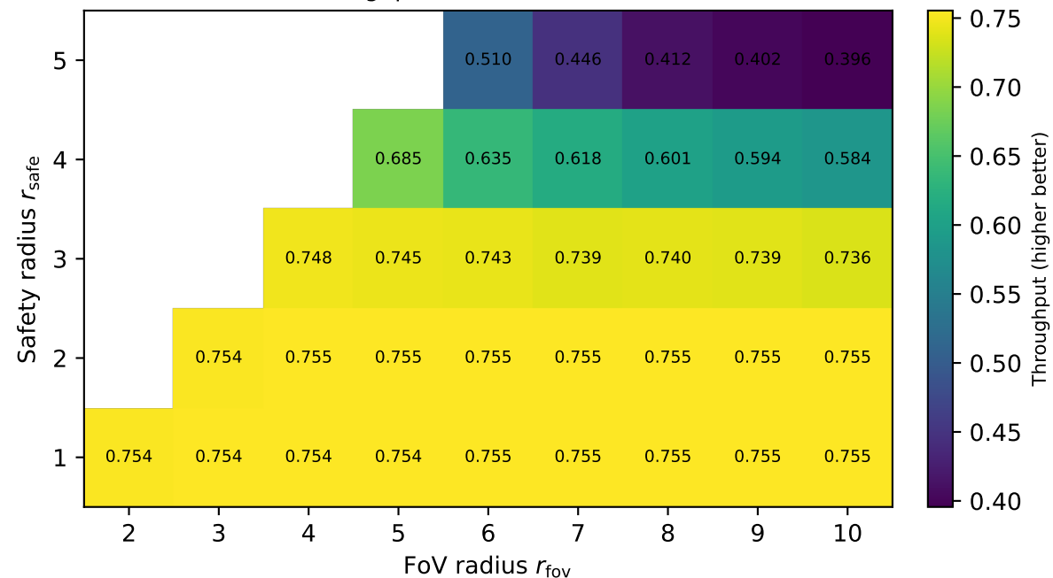
Throughput — random-64-64-10
