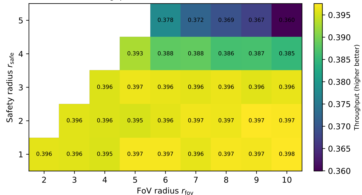
Throughput — warehouse-10-20-10-2-2
