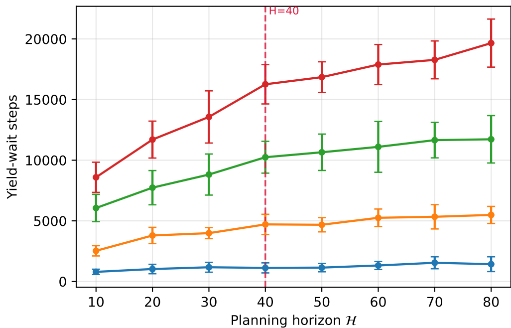
warehouse-10-20-10-2-2
