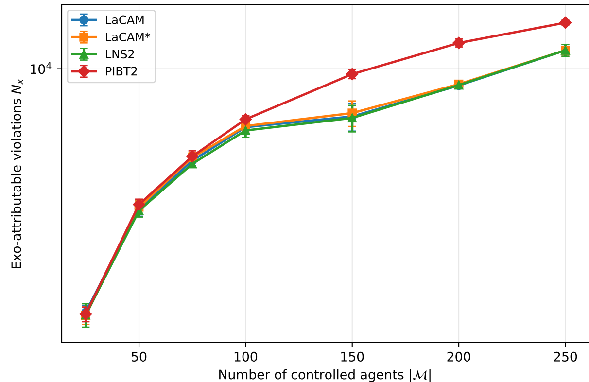
random-64-64-10: scaling_agents @ ( r_{fov} = 3 , r_{safe} = 1 )
