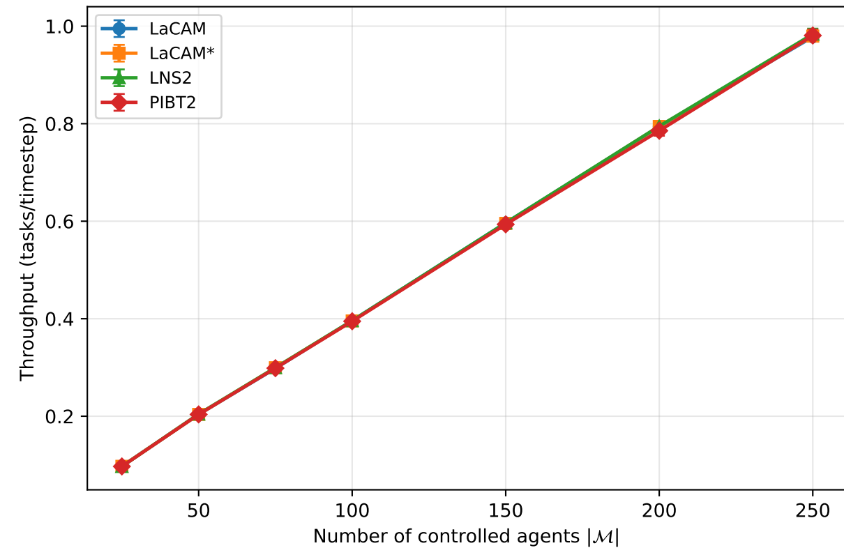
warehouse-10-20-10-2-2: scaling_agents @ ( r_{fov} = 3 , r_{safe} = 1 )
