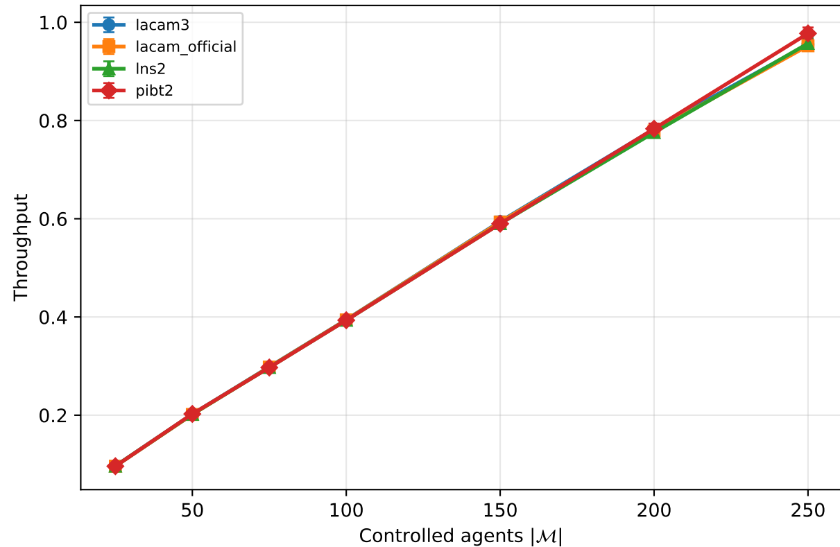
warehouse-10-20-10-2-2
