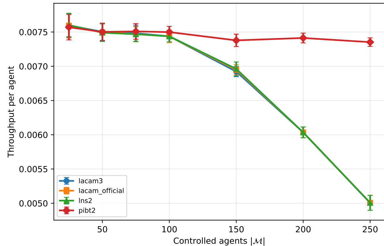
random-64-64-10: agent scaling detail @ ( r_{fov} = 4 , r_{safe} = 2 )
