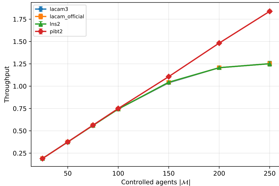
random-64-64-10: agent scaling detail @ ( r_{fov} = 4 , r_{safe} = 2 )
