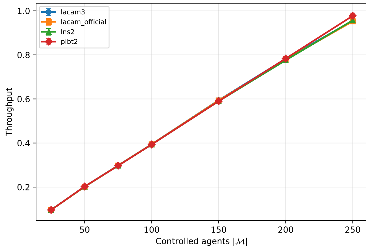
warehouse-10-20-10-2-2: agent scaling detail @ ( r_{fov} = 4 , r_{safe} = 2 )
