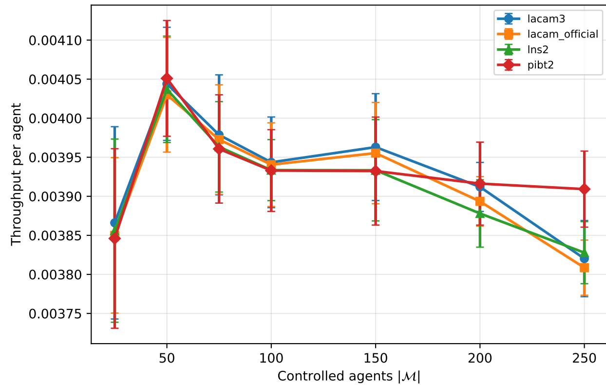
warehouse-10-20-10-2-2: agent scaling detail @ ( r_{fov} = 4 , r_{safe} = 2 )
