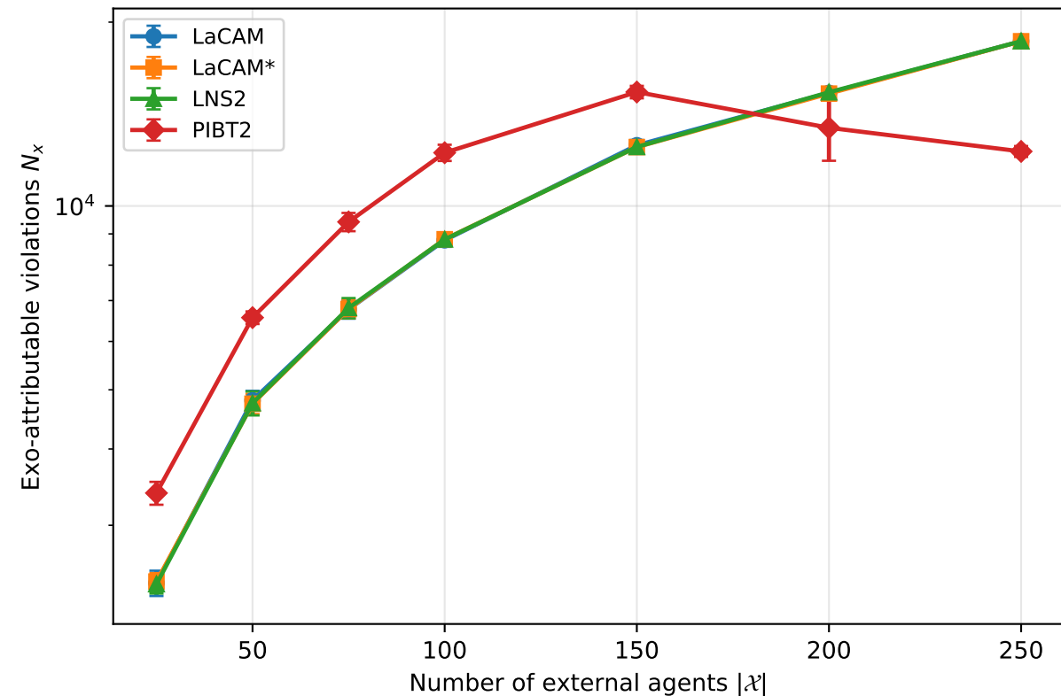
random-64-64-10: scaling_humans @ ( r_{fov} = 3 , r_{safe} = 1 ), |\mathcal{M}| = 200
