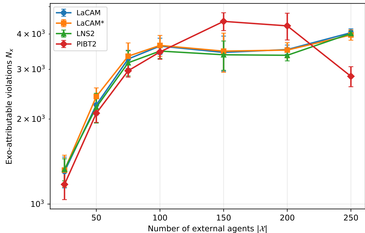
warehouse-10-20-10-2-2: scaling_humans @ ( r_{fov} = 3 , r_{safe} = 1 ), |\mathcal{M}| = 200
