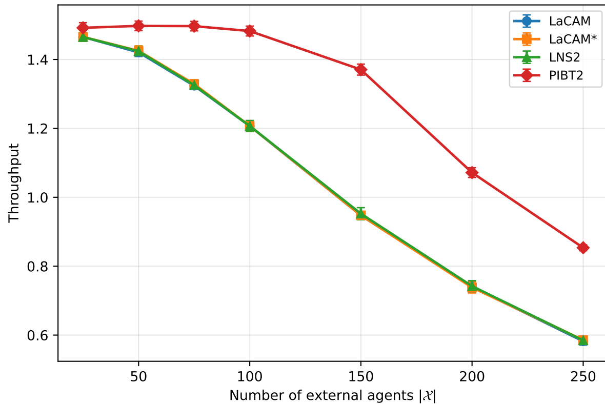
random-64-64-10: scaling_humans @ ( r_{fov} = 4 , r_{safe} = 2 ), |\mathcal{M}| = 200
