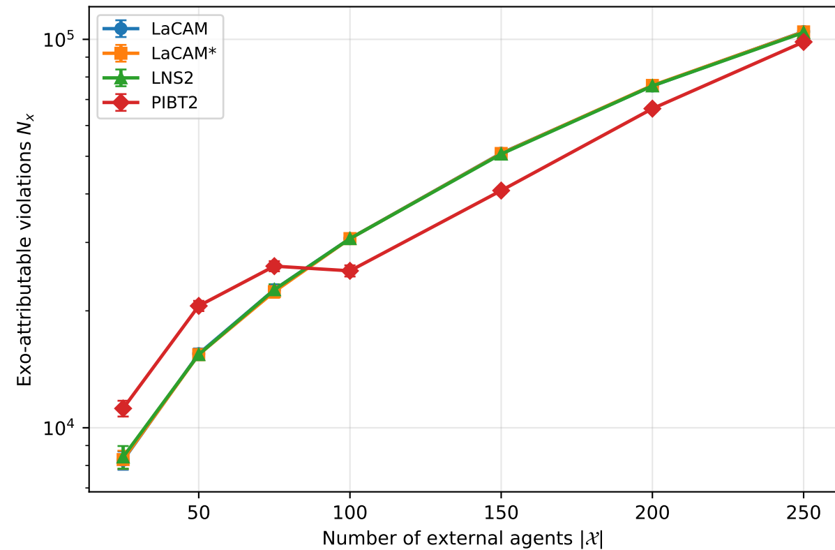
random-64-64-10: scaling_humans @ ( r_{fov} = 4 , r_{safe} = 2 ), |\mathcal{M}| = 200
