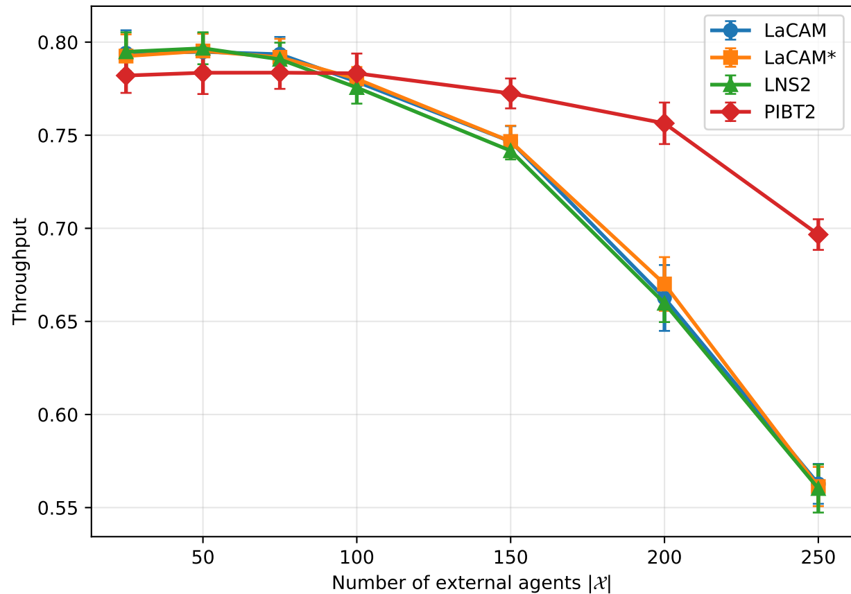
warehouse-10-20-10-2-2 ( |\mathcal{M}| = 200 , r_{fov} = 4 , r_{safe} = 2 )
