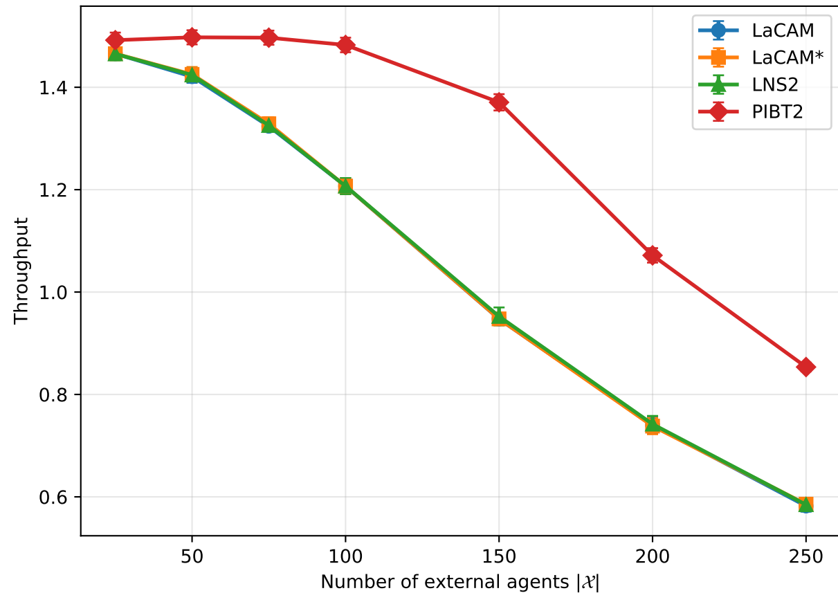
random-64-64-10 ( |\mathcal{M}| = 200 , r_{fov} = 4 , r_{safe} = 2 )
