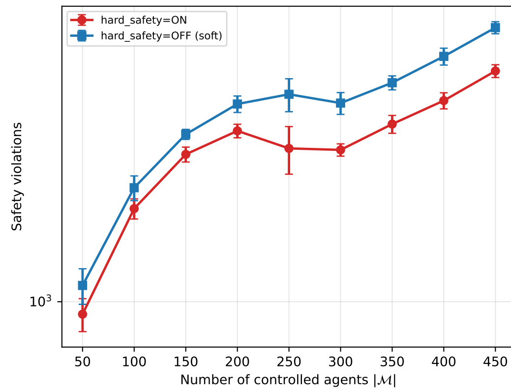
Soft-safety ablation @ warehouse-10-20-10-2-2 (congestion_avoidance, lacam_official, 100 humans)
