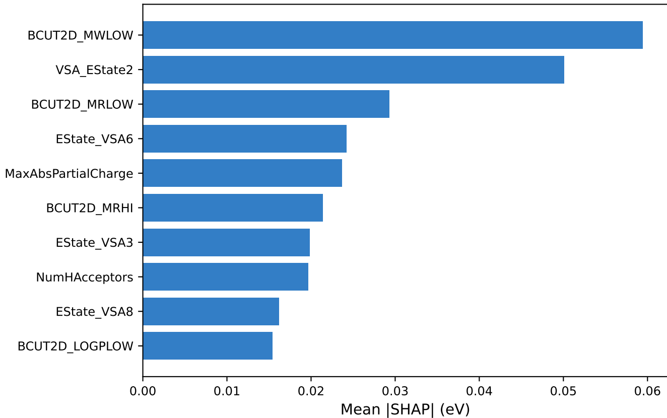
LUMO Feature Importance
