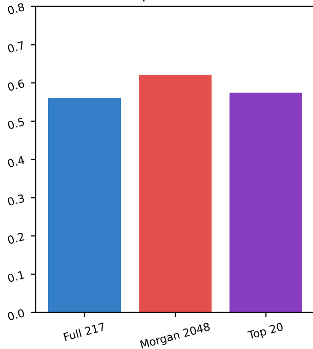
Gap LOOCV R^2
