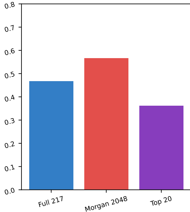
HOMO LOOCV R^2
